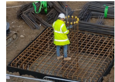
Construction of pile caps
